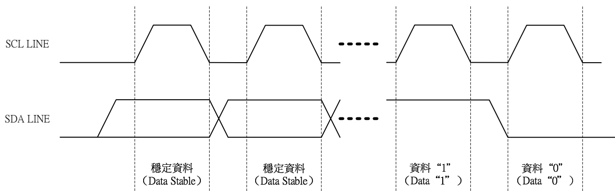
Figure 10 Valid Data Wave Form of Communication I 2 C
