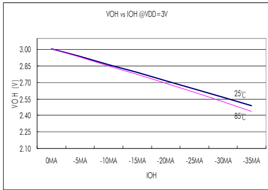
Figure 6.4-1 V_{OH} vs. I_{OH} @VDD=3.0V
