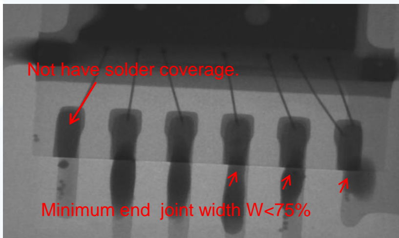
Incomplete reflow of solder paste
