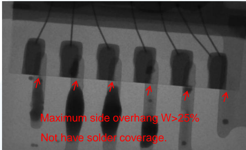
Nonwetting & insufficient solder
