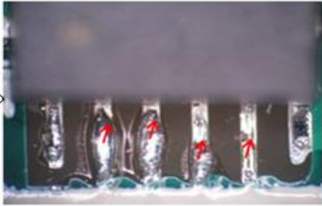
Nonwetting & insufficient solder
