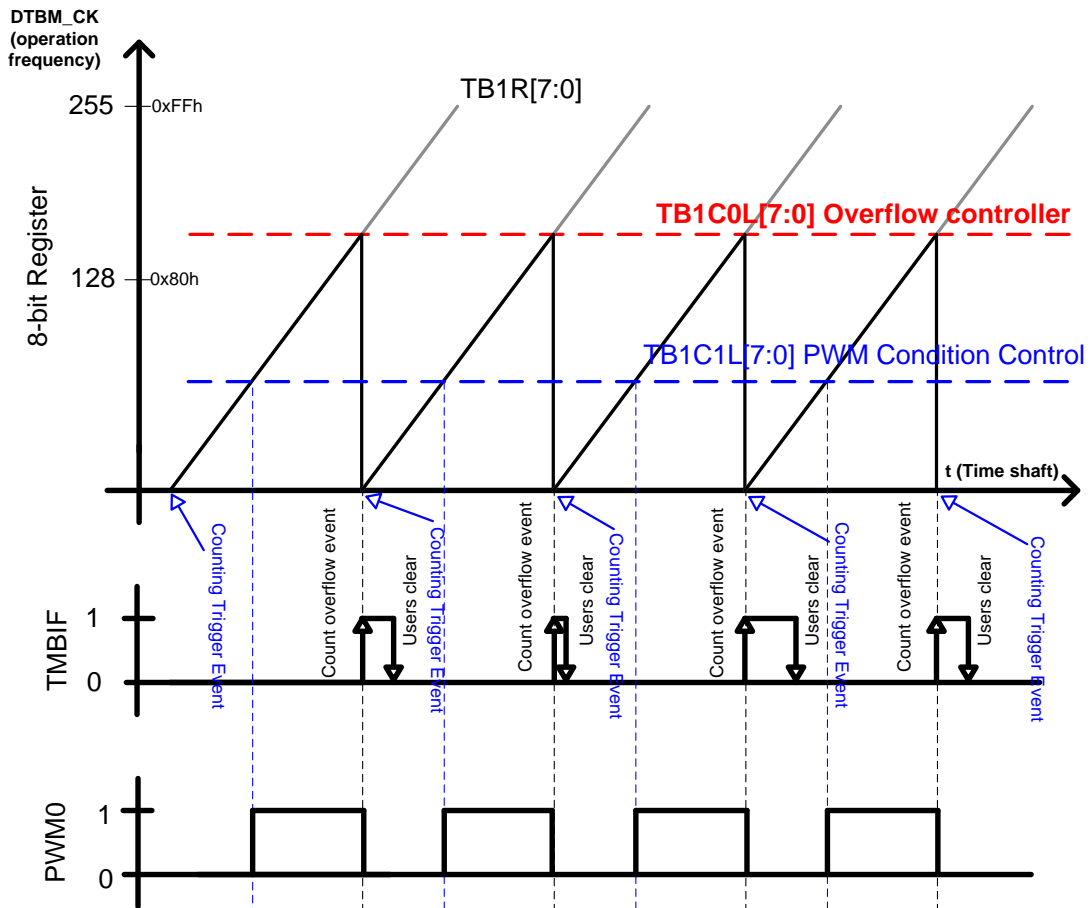
Figure 8-4 PWM1 Waveform and Using Schematic Diagram
