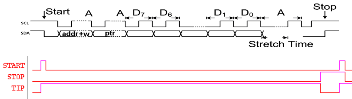
Figure 12-1 I 2 C Bus timing diagram
