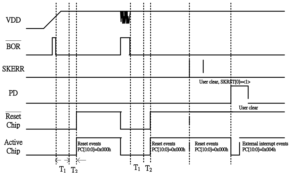
Figure 4-2 Sequence Diagram of Reset & Operation Mode and Status Flags
