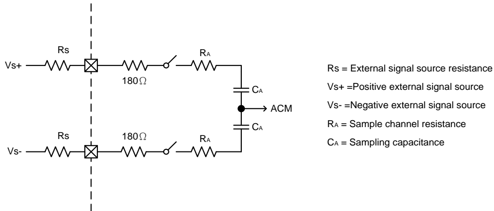
Figure 10-4 AIx Input Capatitor and Impedance Module
