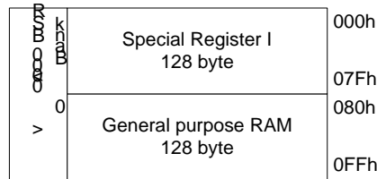
Figure 2-3 Data Memory (DM) Architecture
