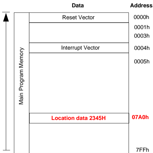
Program Memory Size Table 2KW : PC[10:0]
