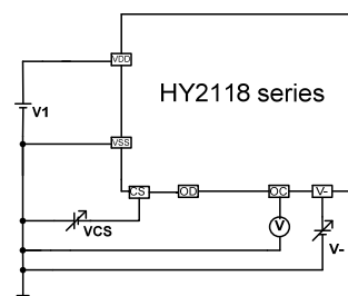
Test circuit 4
