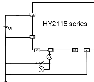
Test circuit 10
