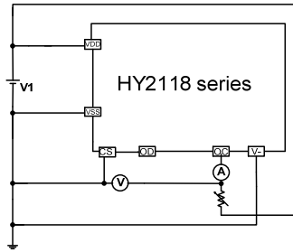
Test circuit 13
