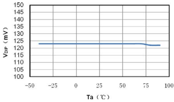
(7) V_{DIP} vs. T_a
